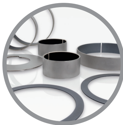
SELF-LUBRICATING CUSTOM-MADE BEARINGS AND BUSHES TX, TF and PMT - Bearings and bushing in any size, in various metals and alloys
