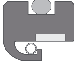
Lipseals sizes according DIN 3760
